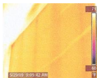
4" Studs / 16" O.C. ½" Sheetrock ¾" Strapping / Furring ¾" Thermal 3Ht R-11 Fiberglass 7/16" OSB R-Value 19.5
